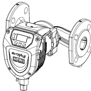
Figure 2: Installation on horizontal pipes
